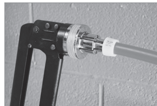
6. Expand by pressing the tool handles together. Open handles, rotate tool and repeat. Refer to the chart below for the recommended number of expansions per tubing size.
