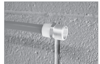
8. Immediately remove the tool from the pipe and sleeve. Insert the fitting until its shoulder touches the sleeve end. Pipe may take up to two minutes to fully seal fitting.
