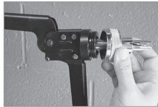
2. Attach the expansion head onto the expansion tool.
