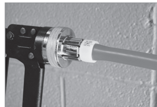
7. Expansion is complete when the pipe and sleeve are against the shoulder of the tool head.
