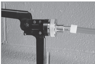
5. Open the tool handles fully and gently insert the tool head into pipe until it stops.
